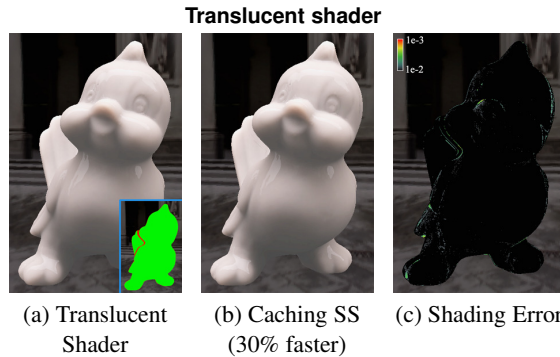
Figure 8: A translucent shader based on PRT [WTL05] accelerated with our caching strategy. (a) One frame from a sequence in which the user adjusts the position of the bird model under environment lighting. (b) Result of caching and reusing the single-scattering shading calculation (note the cache is never explicitly refreshed as seen in the coherence map in (a,cutout)).
