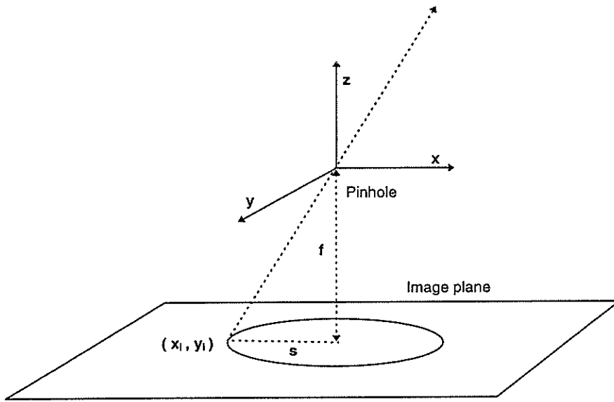
Figure 1: Camera geometry
