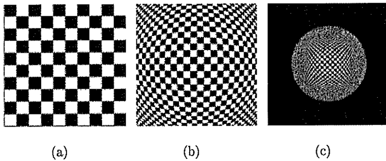
Figure 6: Infinite plane. (a) \beta = 0.00 ; (b) \beta = 0.50 ; (c) \beta = 0.90
