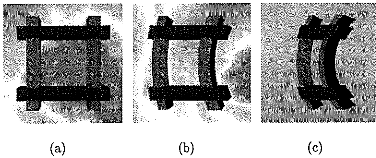
Figure 8: Simple grid, looking sideways. (a) \beta = 0.00, \Delta x' = 0 ; (b) \beta = 0.50, \Delta x' = 1.73 ; (c) \beta = 0.90, \Delta x' = 9.17
